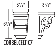
7" CELTIC CORBEL R•26
