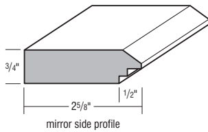
mirror side profile
