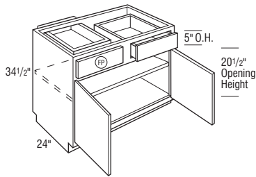
Peninsula Side Shown
