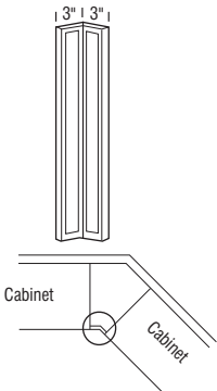
Installation of 1350FW, 1350F029 and 1350FB (overhead view)
