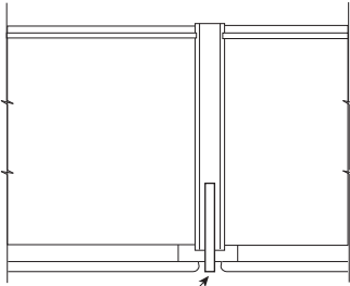
PIL530 pilaster w/TBEM
