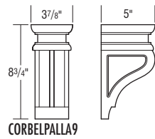
9" PALLADIAN CORBEL R•25
