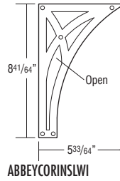
ABBEY CORBEL INSERT - LARGE R•28
