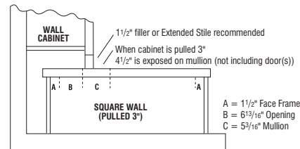
Top View Full Overlay Styles, Pulled 3"
