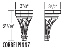
7" PINNACLE CORBEL R•26
