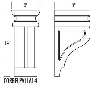
14" PALLADIAN CORBEL R•25
