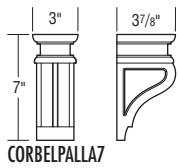
7" PALLADIAN CORBEL R•25
