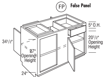
BCFW48P L or R Left Shown
