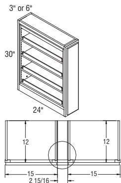
Top View Installation
