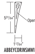
ABBEY CORBEL INSERT - MEDIUM R•28
