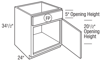
FP False Panel
