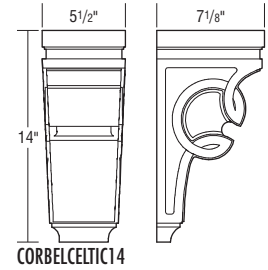
14" CELTIC CORBEL R•26
