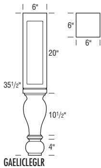
GAELIC LEG, LARGE, ROUTED R•41
