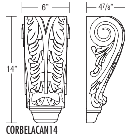
14" SMALL ACANTHUS CORBEL R•27
