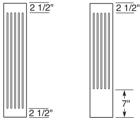
Wall/Base Base with Flush Toe Kick Option
