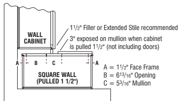
Top View Full Overlay Styles
