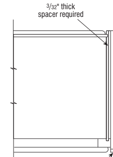
PIL W30 pilaster w/TBEM
