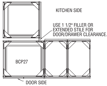
OTHER ROOM SIDE Top View
