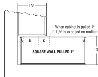
Top View Inset Styles, Pulled 1"
