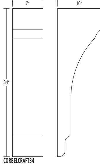
34" CRAFTSMAN CORBEL R•25
