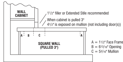
Top View Full Overlay Styles, Pulled 3"
