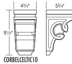
10" CELTIC CORBEL R•26
