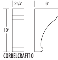
10" CRAFTSMAN CORBEL R•25
