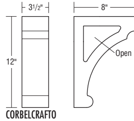
CRAFTSMAN CORBEL OPEN R•24
