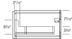
Top U-shaped drawer box has cascading side drawer feature.
