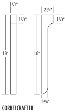
18" CRAFTSMAN CORBEL R•25
